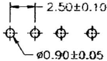
PCB LAYOUT
