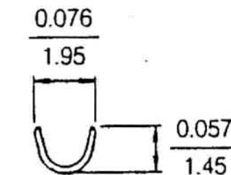
SECT B-B
